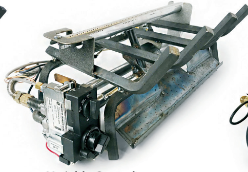
Variable Control with Burner & Remote
